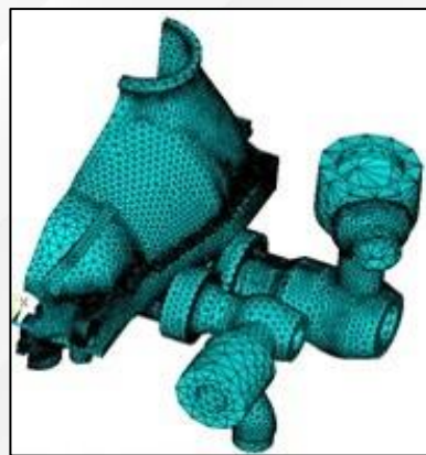
3D Finite Element Meshing
